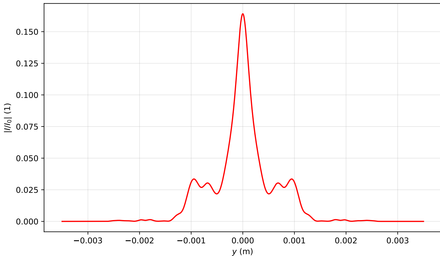
Intensity profile I(x=0, y, z=2.866)/I_0 , P_{in}=15.0\text{Pcr} , artificial time
