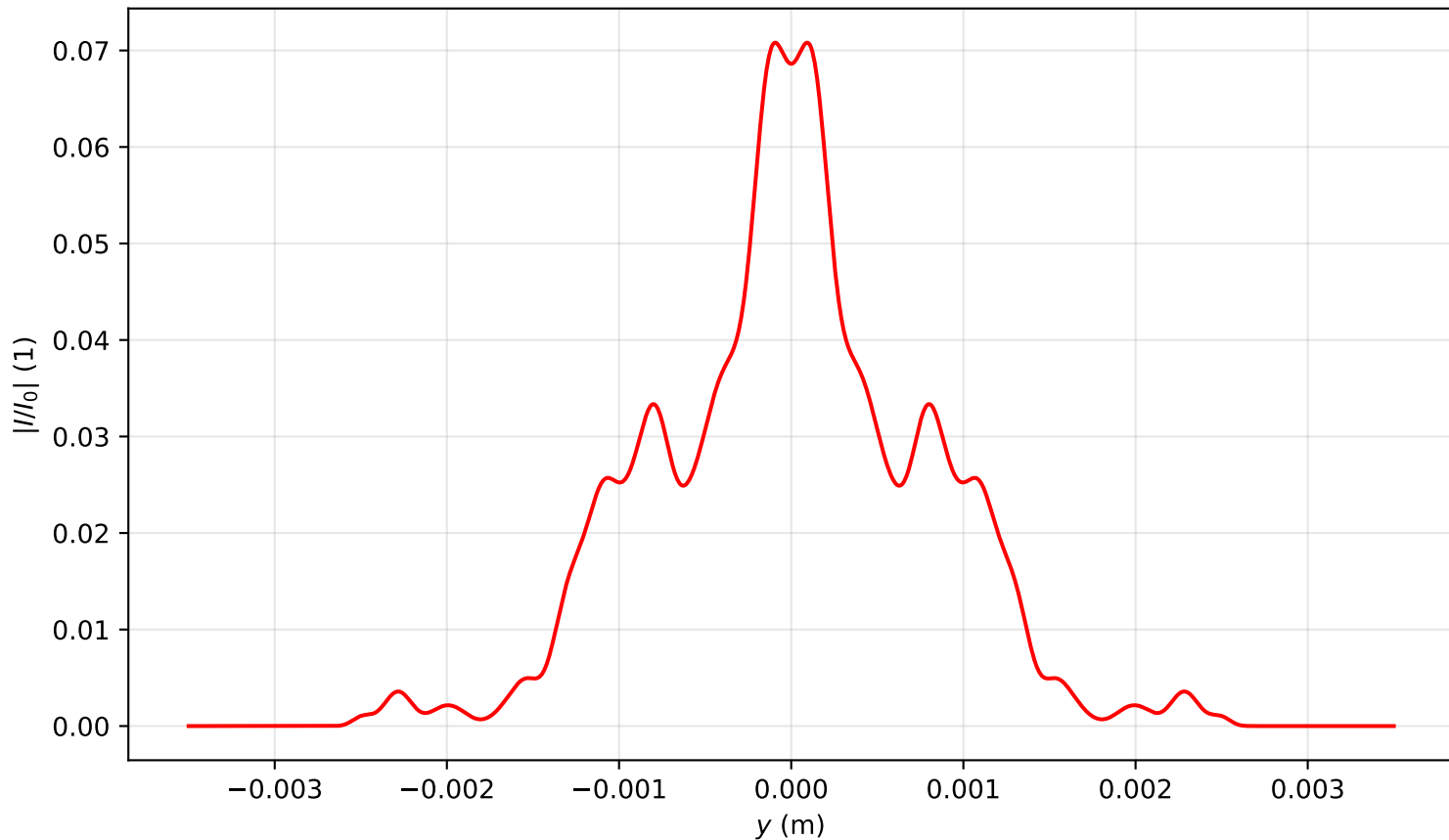
Intensity profile I(x=0, y, z=3.105)/I_0 , P_{in}=15.0\text{Pcr} , artificial time
