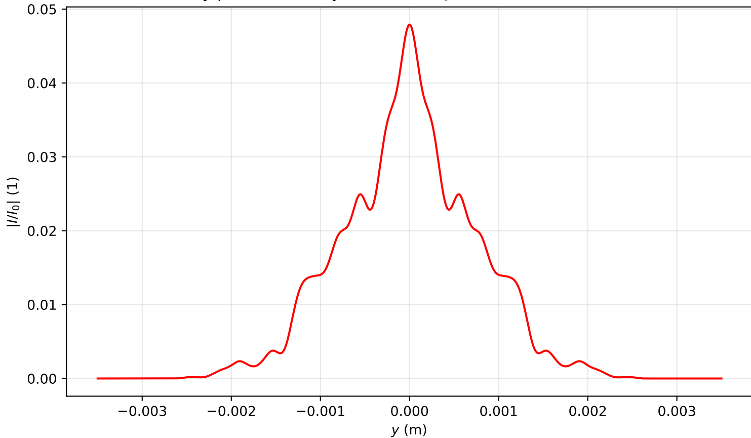
Intensity profile I(x=0, y, z=3.344)/I_0 , P_{in}=15.0\text{Pcr} , artificial time
