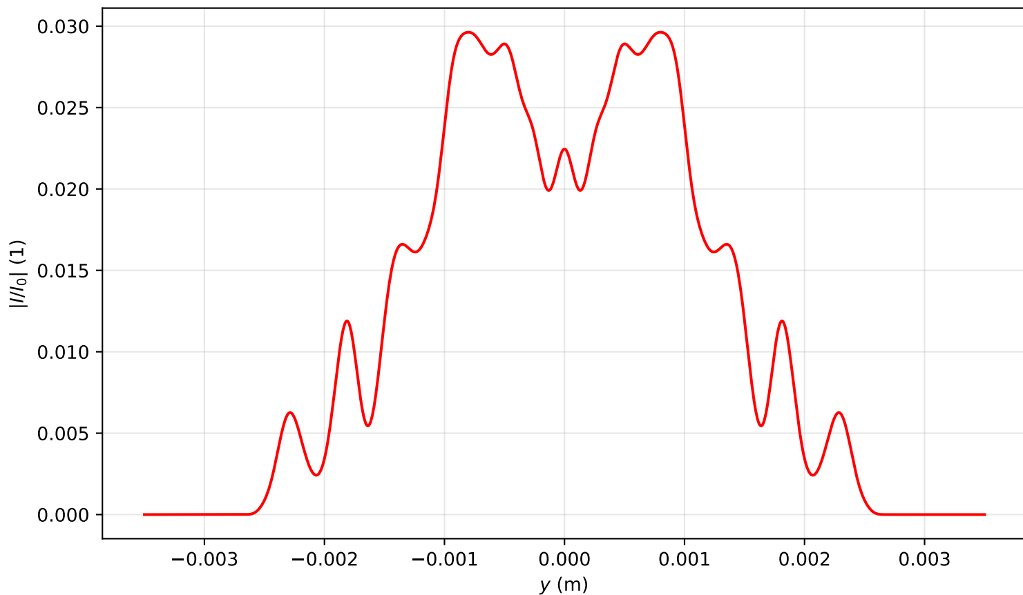
Intensity profile I(x=0, y, z=3.582)/I_0 , P_{in}=15.0P_{cr} , artificial time
