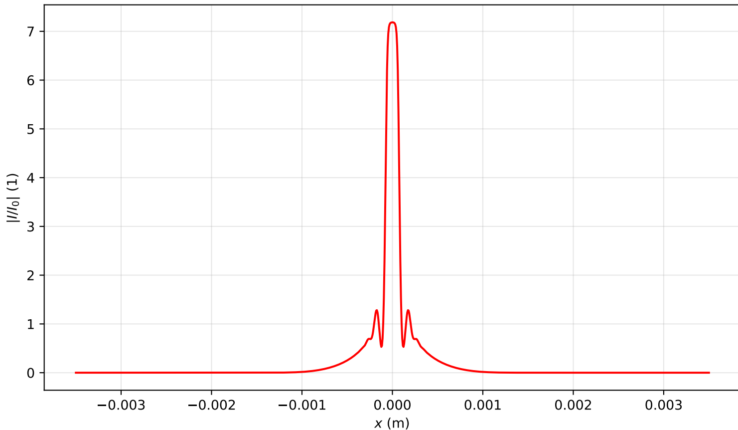
Intensity profile I(x, y = 0, z = 0.239)/I_0 , P_{in}=15.5P_{cr} , artificial time
