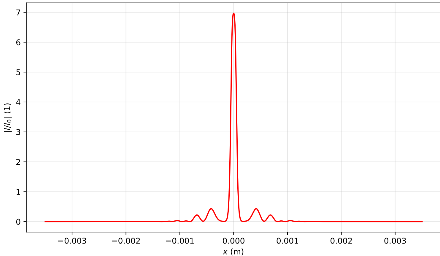
Intensity profile I(x, y = 0, z = 0.716)/I_0 , P_{in}=15.5P_{cr} , artificial time
