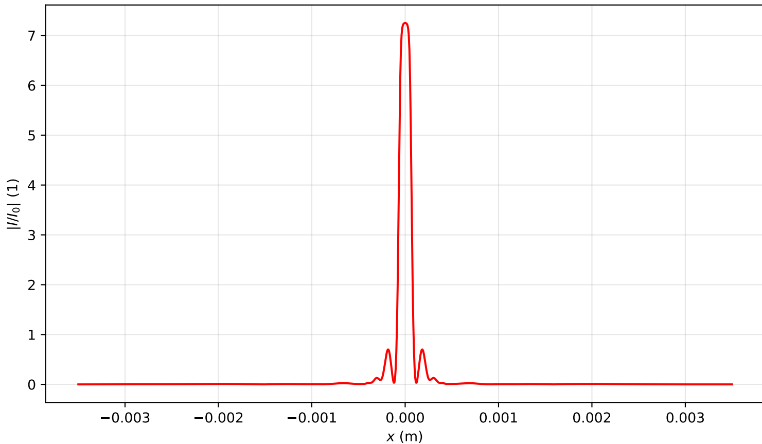
Intensity profile I(x, y = 0, z = 1.433)/I_0 , P_{in}=15.5P_{cr} , artificial time
