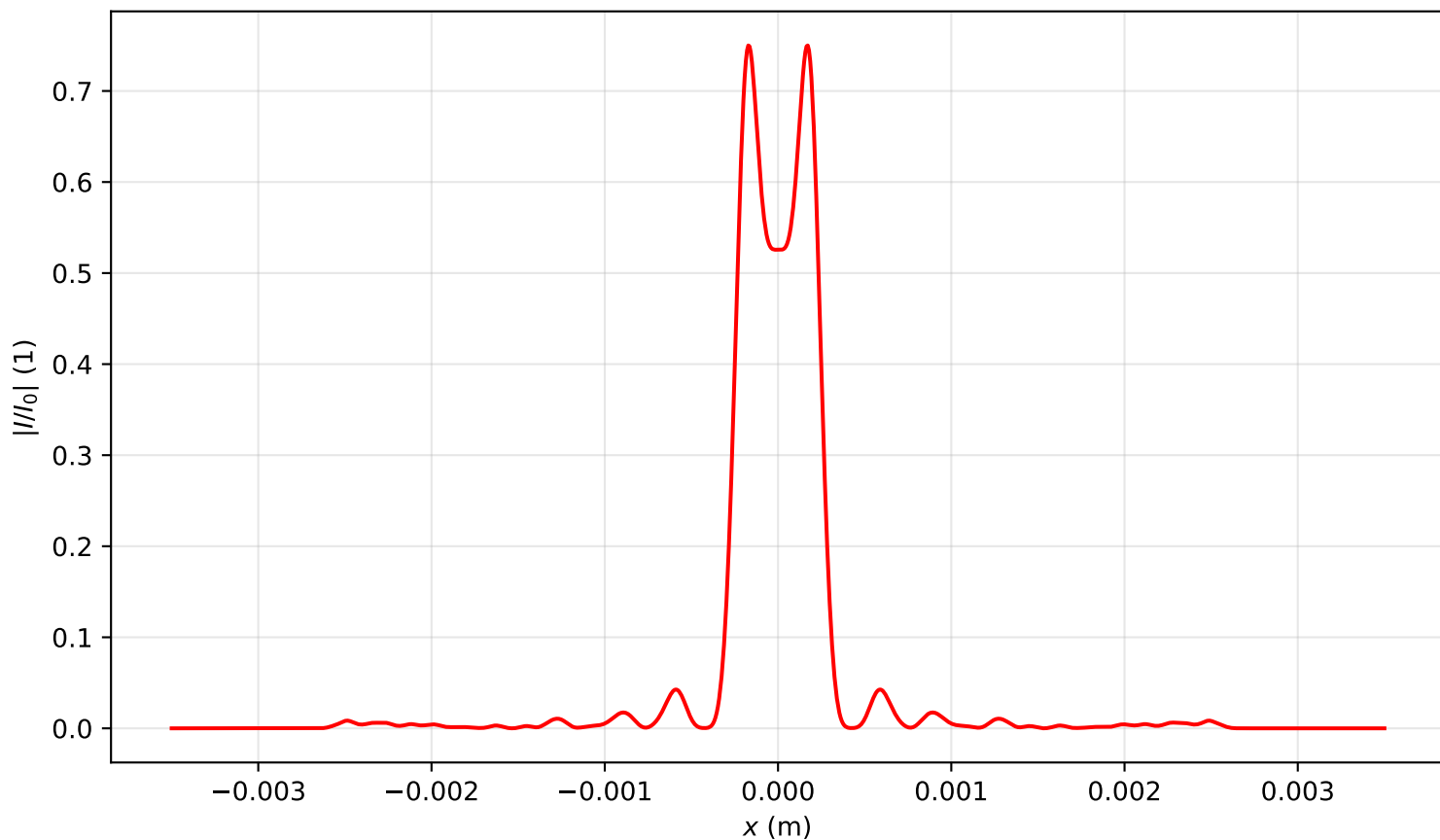
Intensity profile I(x, y = 0, z = 1.672)/I_0 , P_{in}=15.5P_{cr} , artificial time
