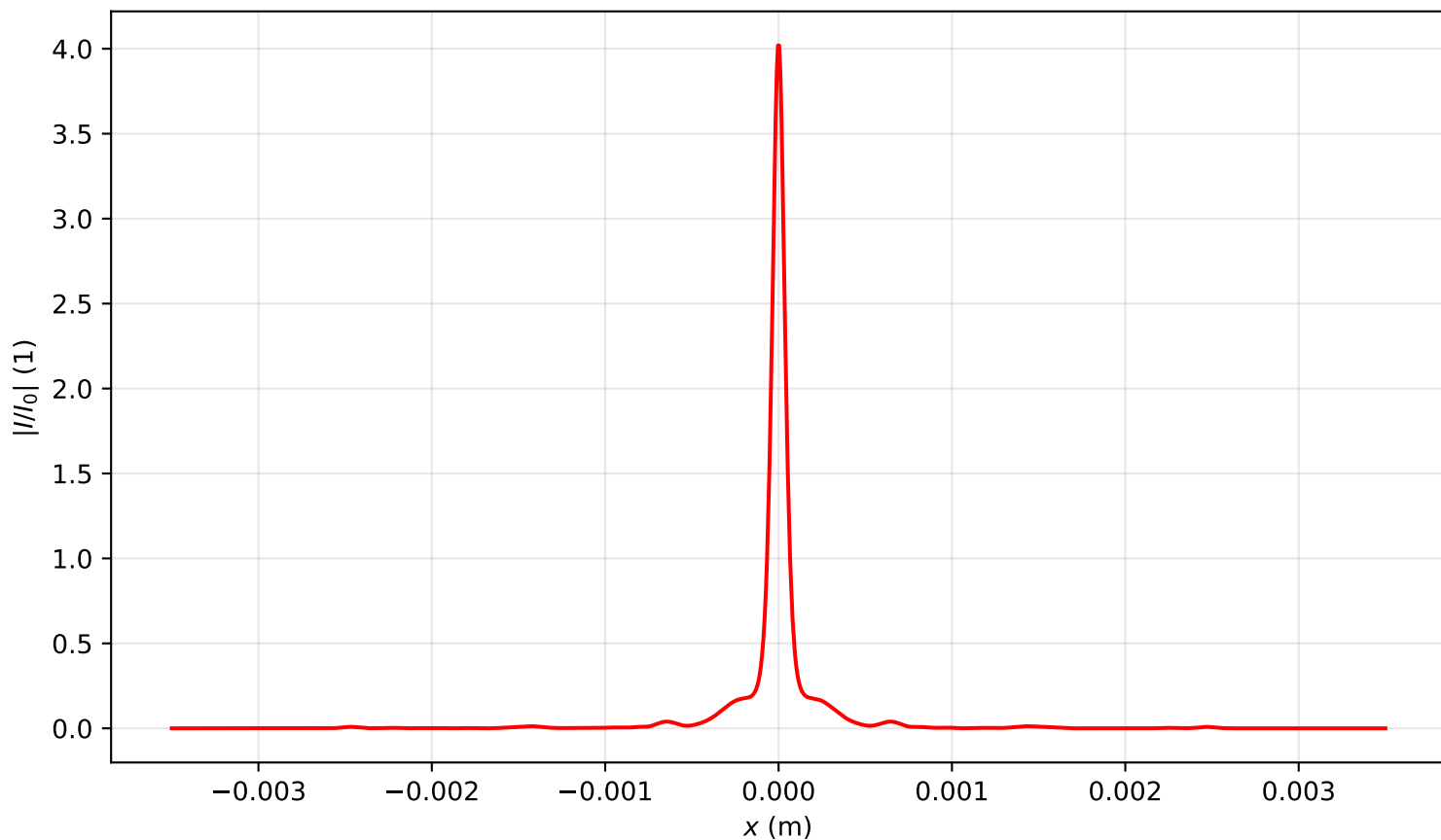
Intensity profile I(x, y = 0, z = 1.911)/I_0 , P_{in}=15.5P_{cr} , artificial time
