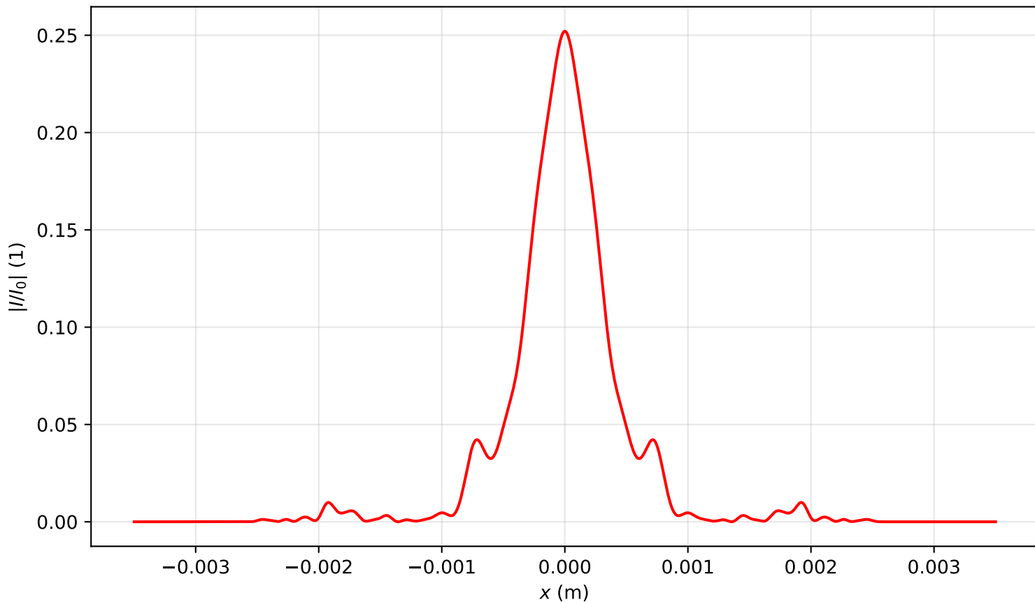
Intensity profile I(x, y = 0, z = 2.149)/I_0 , P_{in}=15.5P_{cr} , artificial time
