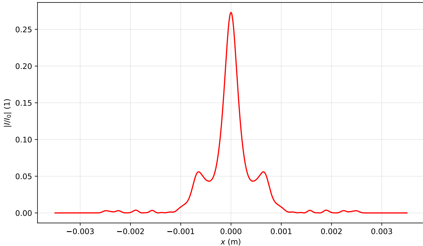
Intensity profile I(x, y = 0, z = 2.388)/I_0 , P_{in}=15.5P_{cr} , artificial time
