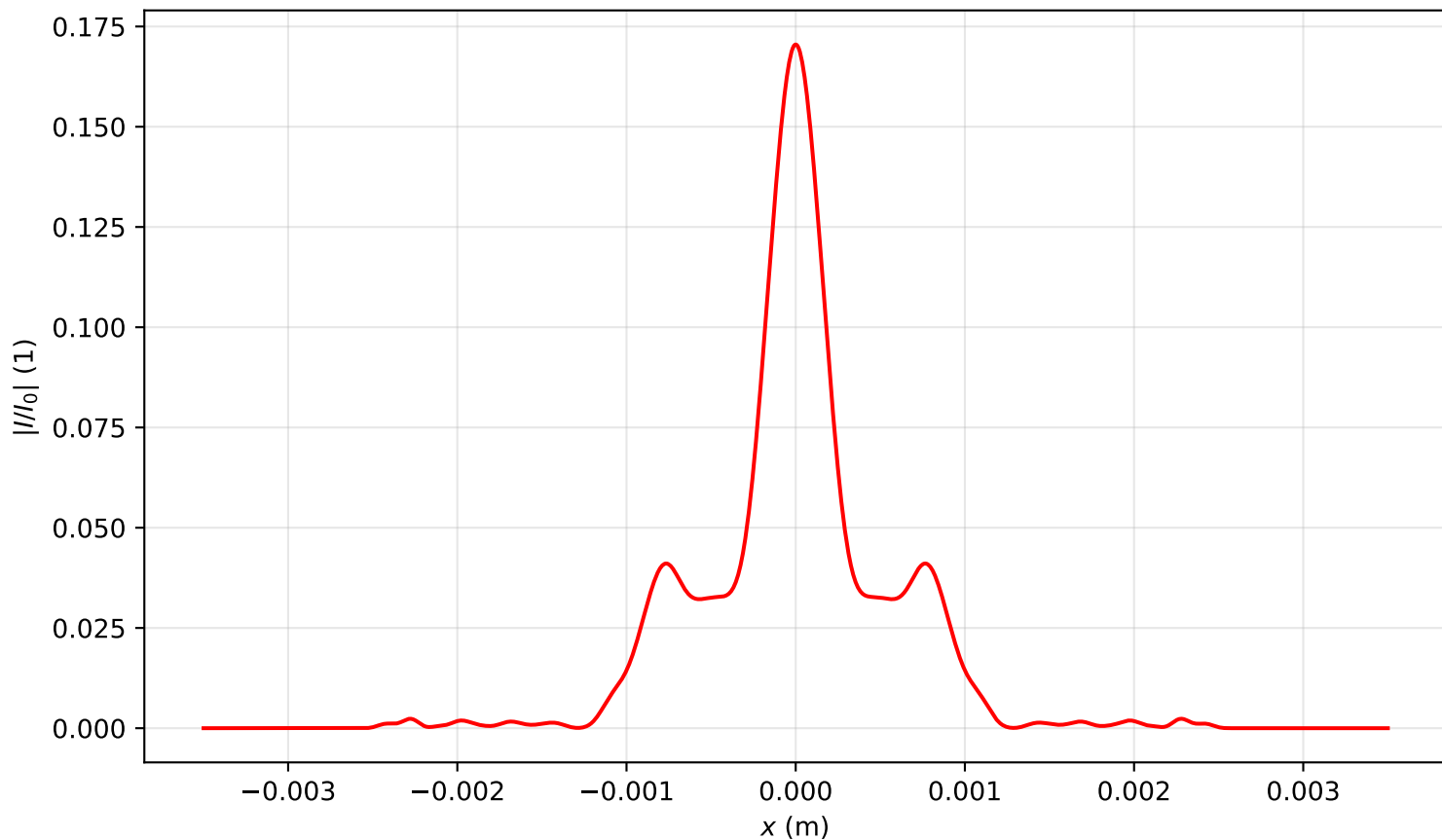
Intensity profile I(x, y = 0, z = 2.627)/I_0 , P_{in}=15.5P_{cr} , artificial time
