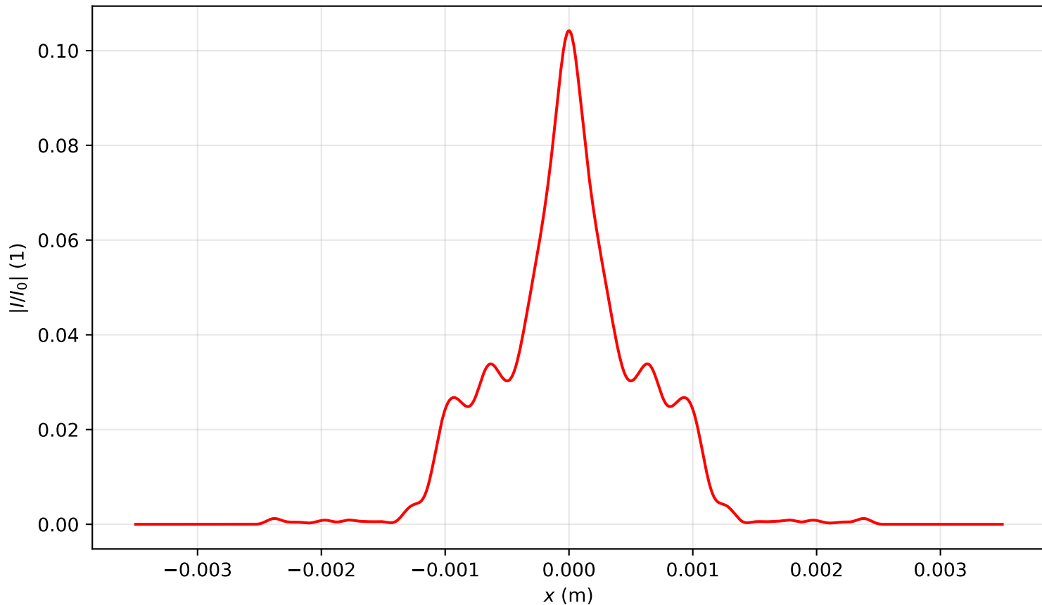
Intensity profile I(x, y = 0, z = 2.866)/I_0 , P_{in}=15.5P_{cr} , artificial time
