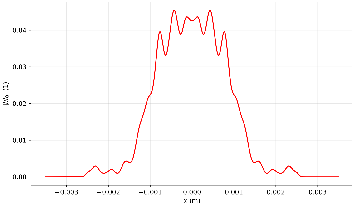
Intensity profile I(x, y = 0, z = 3.105)/I_0 , P_{in}=15.5P_{cr} , artificial time
