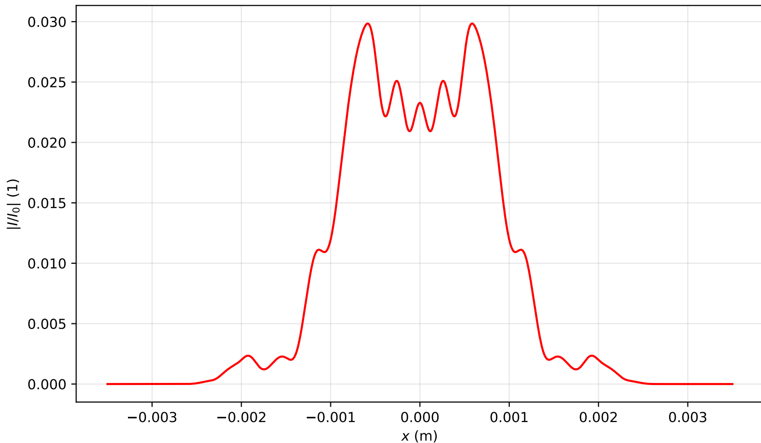
Intensity profile I(x, y = 0, z = 3.344)/I_0 , P_{in}=15.5P_{cr} , artificial time
