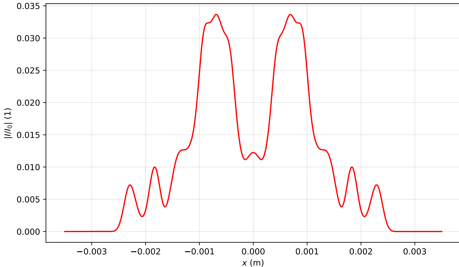
Intensity profile I(x, y = 0, z = 3.582)/I_0 , P_{in}=15.5P_{cr} , artificial time
