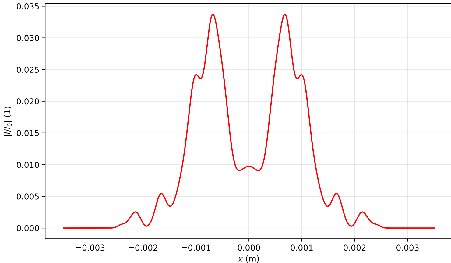
Intensity profile I(x, y = 0, z = 3.821)/I_0 , P_{in}=15.5P_{cr} , artificial time
