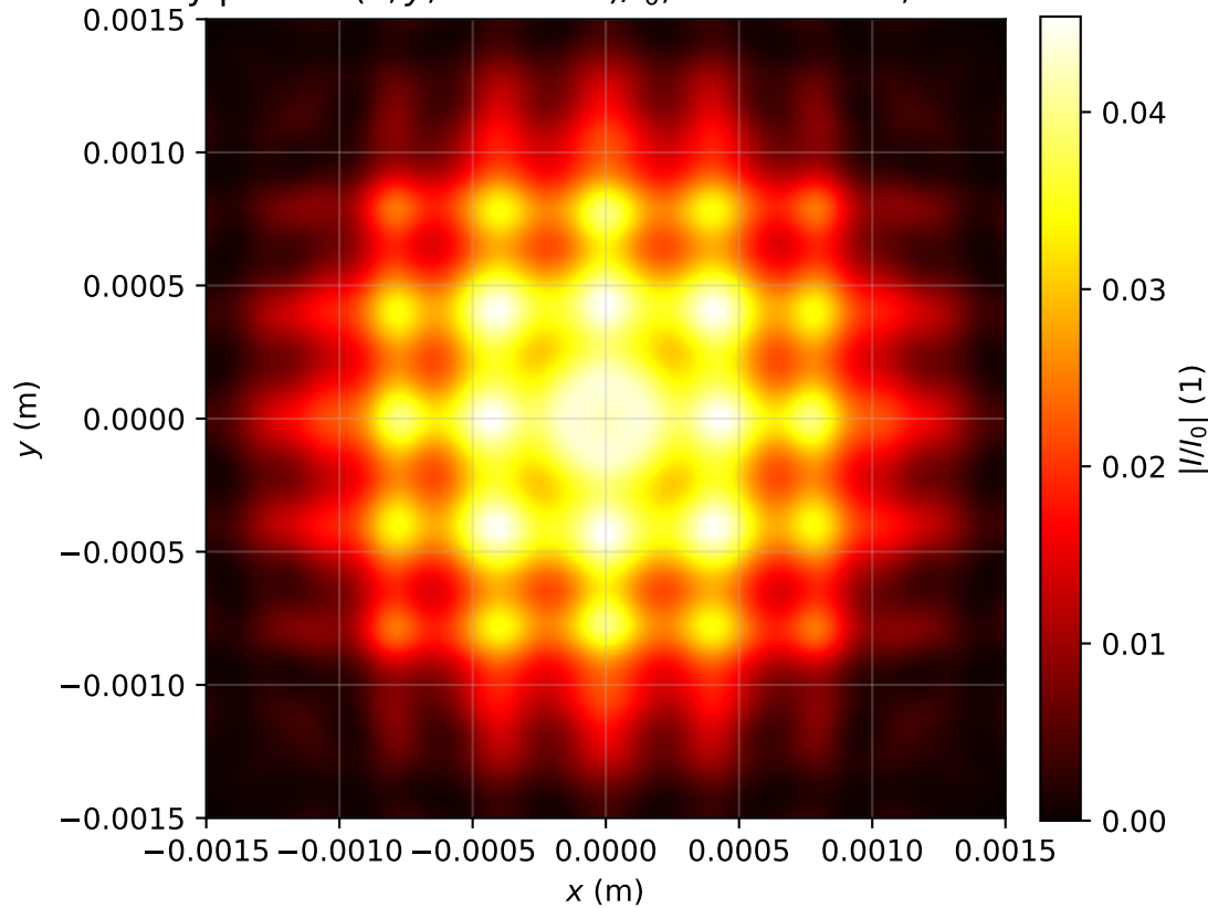
Intensity profile I(x, y, z = 3.105)/I_0 , P_{in}=15.5P_{cr} , artificial time
