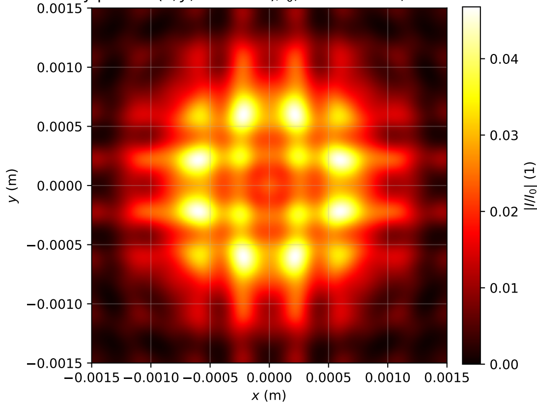
Intensity profile I(x, y, z = 3.344)/I_0 , P_{in}=15.5P_{cr} , artificial time
