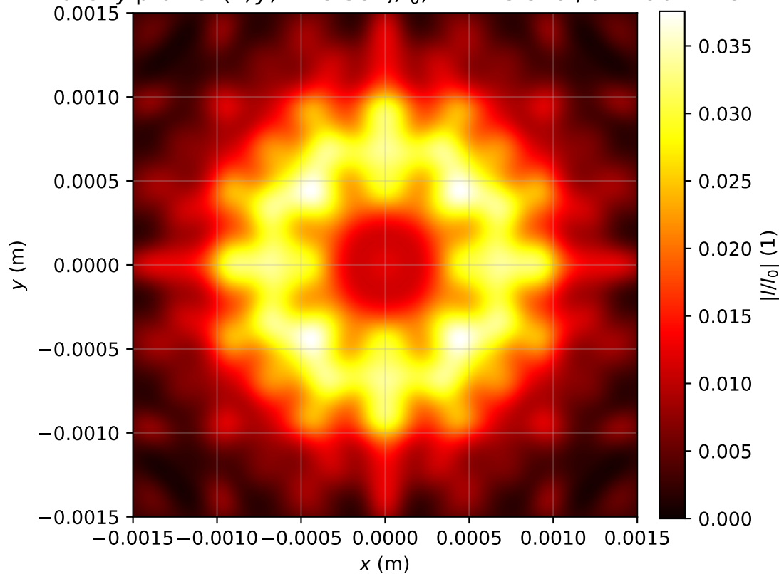
Intensity profile I(x, y, z = 3.582)/I_0 , P_{in}=15.5P_{cr} , artificial time
