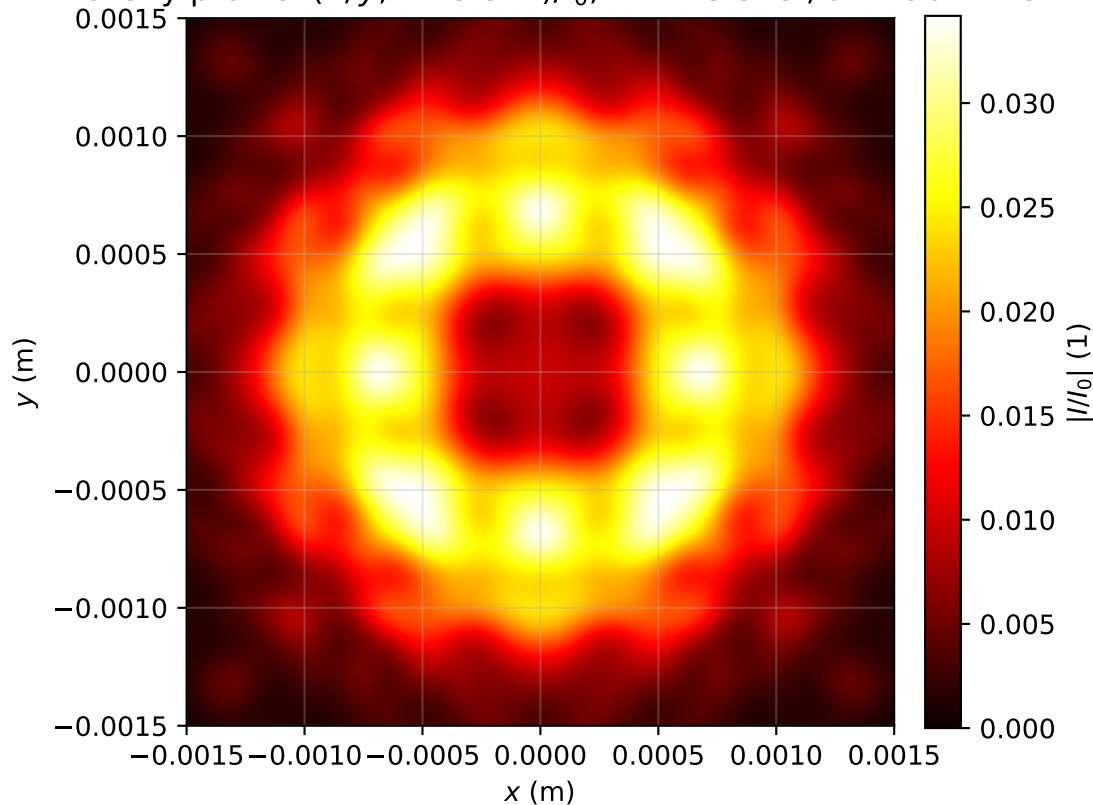
Intensity profile I(x, y, z = 3.821)/I_0 , P_{in}=15.5P_{cr} , artificial time
