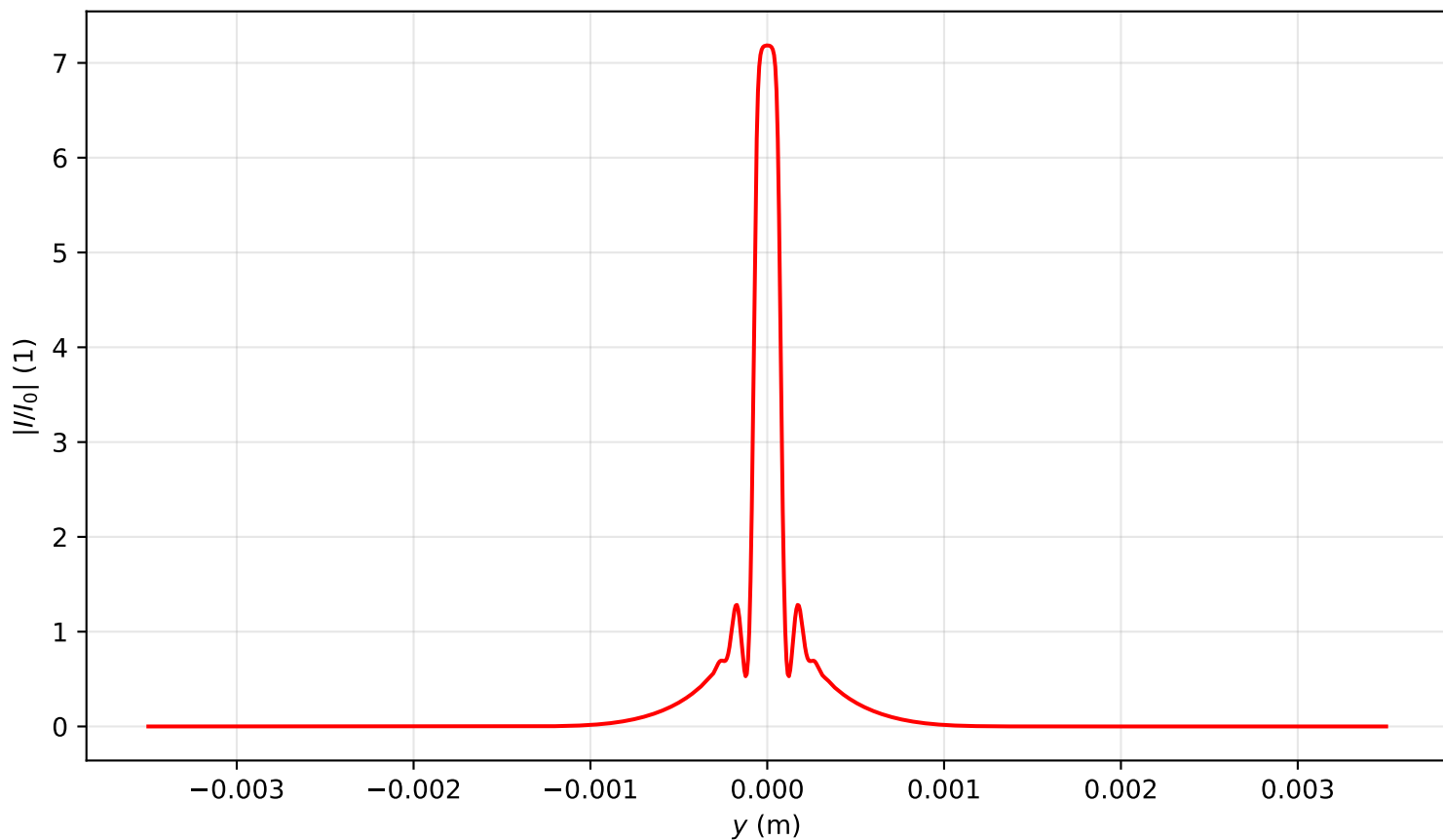
Intensity profile I(x=0, y, z=0.239)/I_0 , P_{in}=15.5P_{cr} , artificial time
