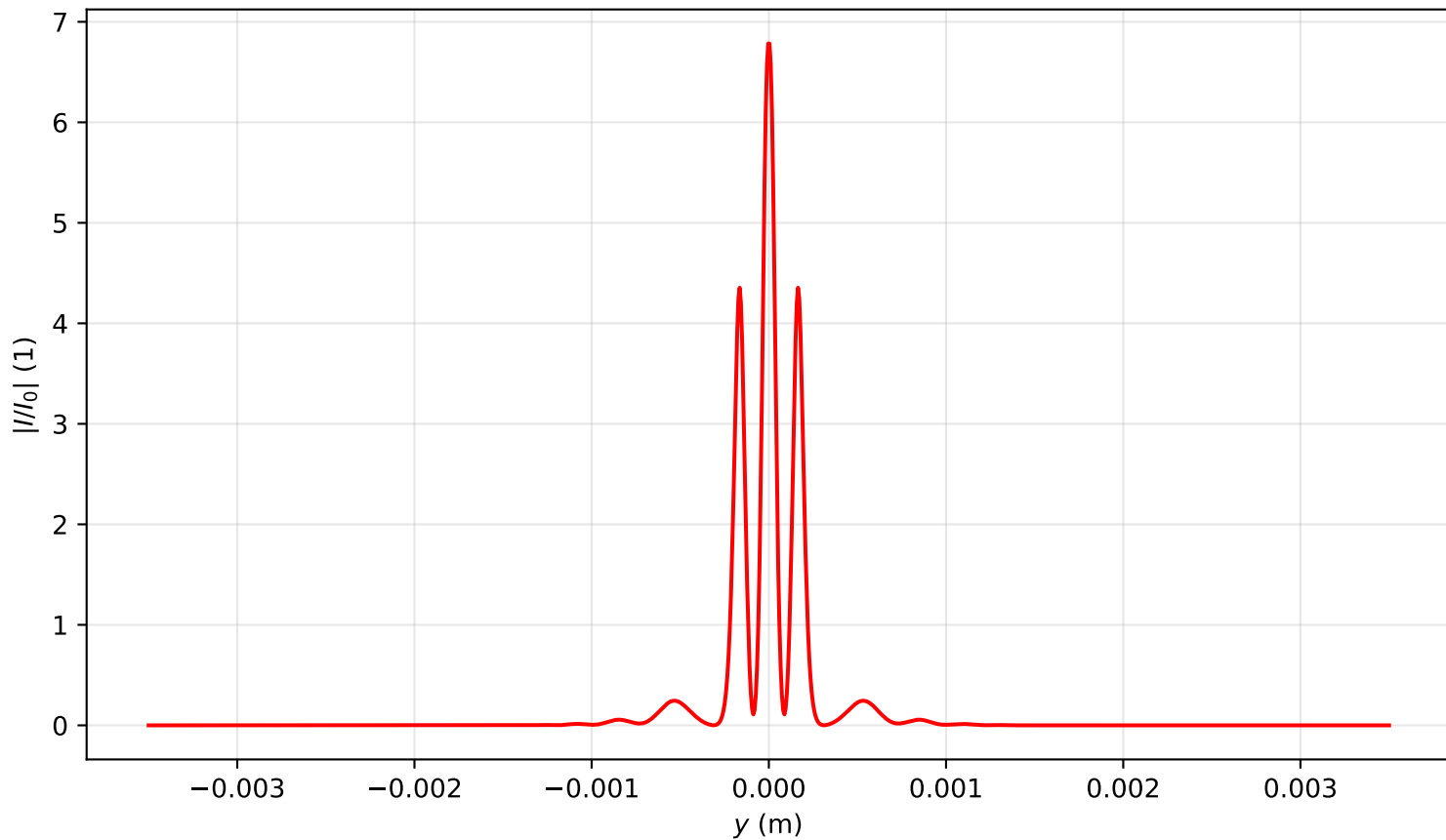
Intensity profile I(x=0, y, z=0.478)/I_0 , P_{in}=15.5P_{cr} , artificial time
