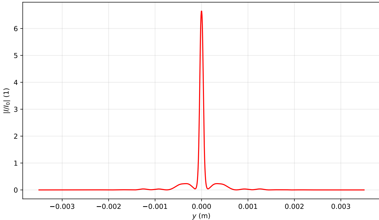
Intensity profile I(x = 0, y, z = 0.955)/I_0 , P_{in}=15.5P_{cr} , artificial time
