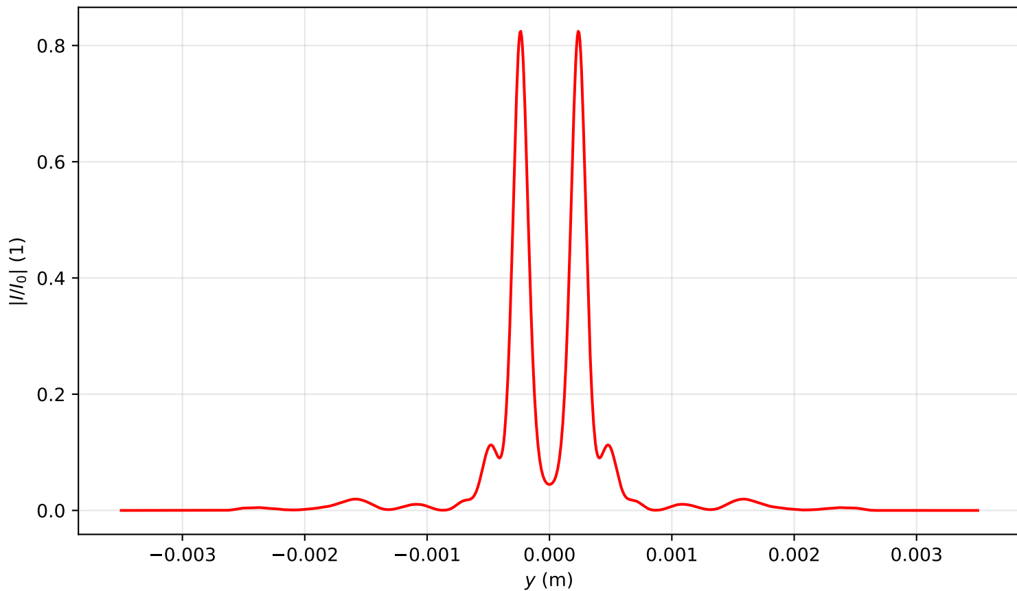
Intensity profile I(x=0, y, z=1.194)/I_0 , P_{in}=15.5P_{cr} , artificial time
