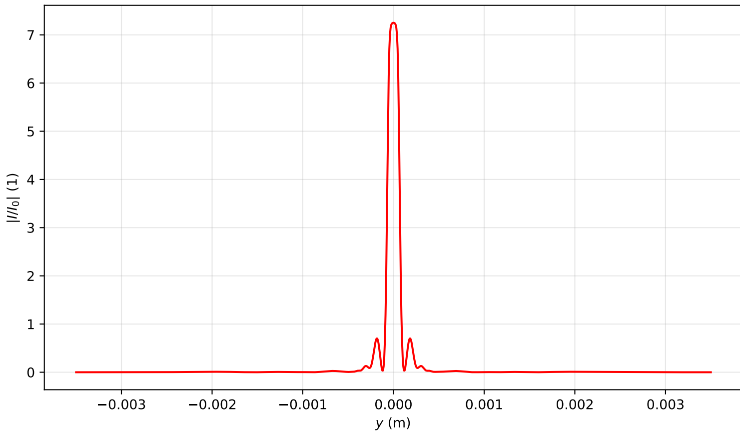
Intensity profile I(x=0, y, z=1.433)/I_0 , P_{in}=15.5P_{cr} , artificial time
