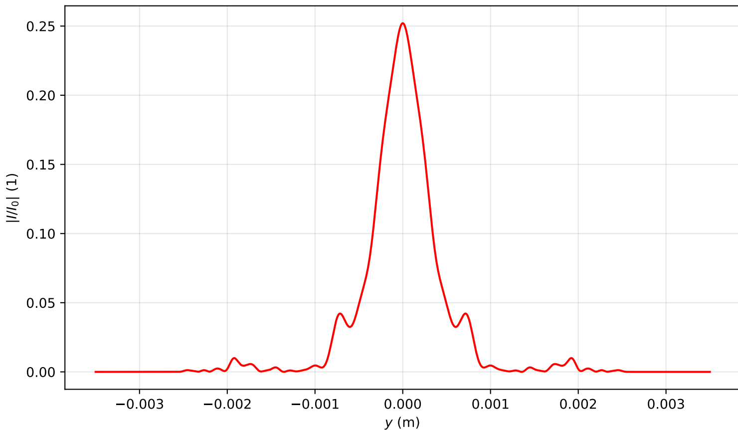
Intensity profile I(x=0, y, z=2.149)/I_0 , P_{in}=15.5P_{cr} , artificial time
