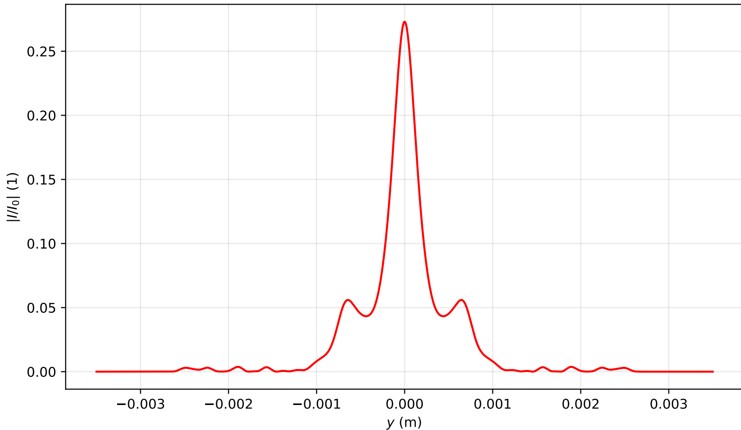
Intensity profile I(x=0, y, z=2.388)/I_0 , P_{in}=15.5P_{cr} , artificial time
