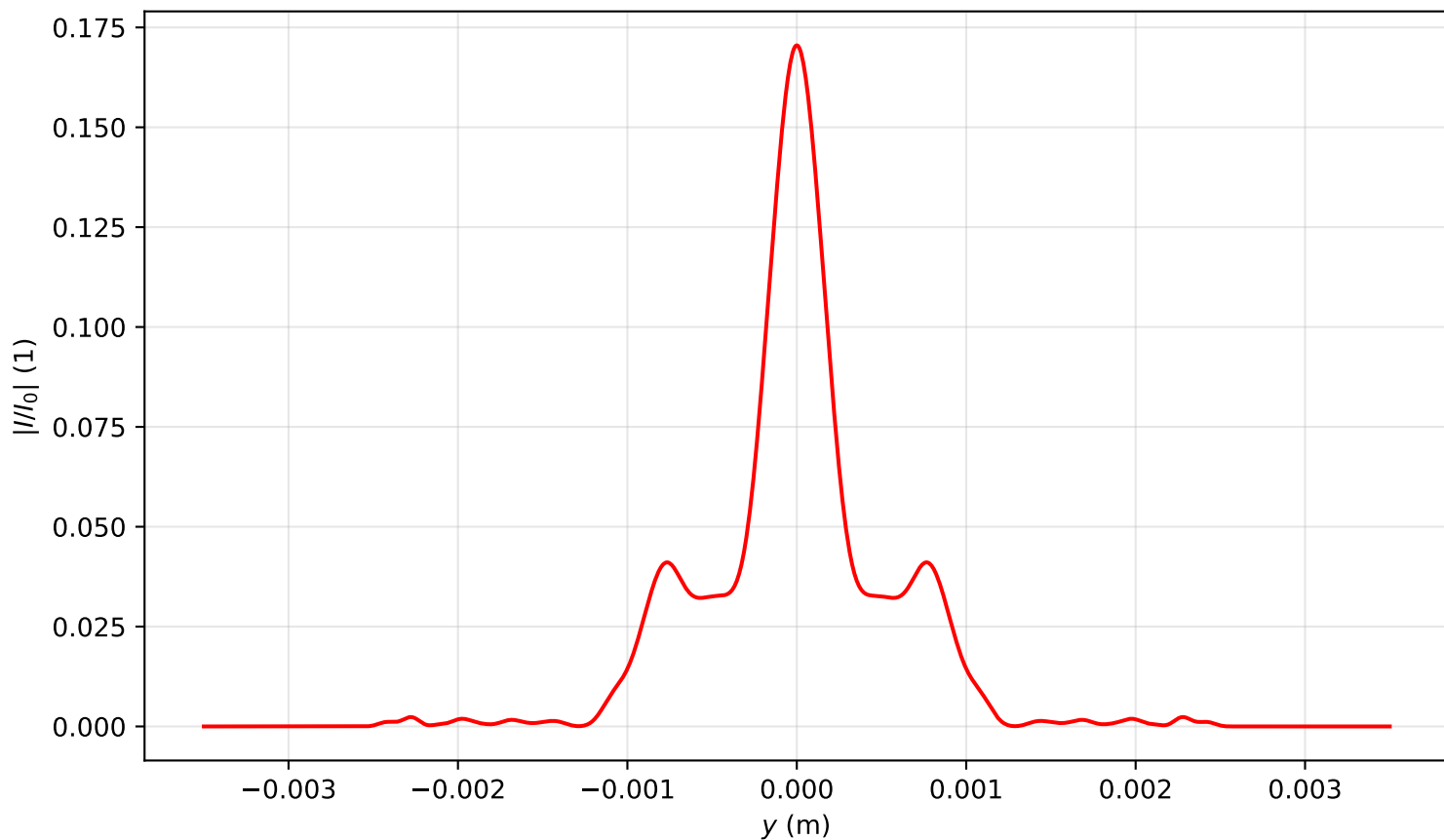
Intensity profile I(x=0, y, z=2.627)/I_0 , P_{in}=15.5P_{cr} , artificial time
