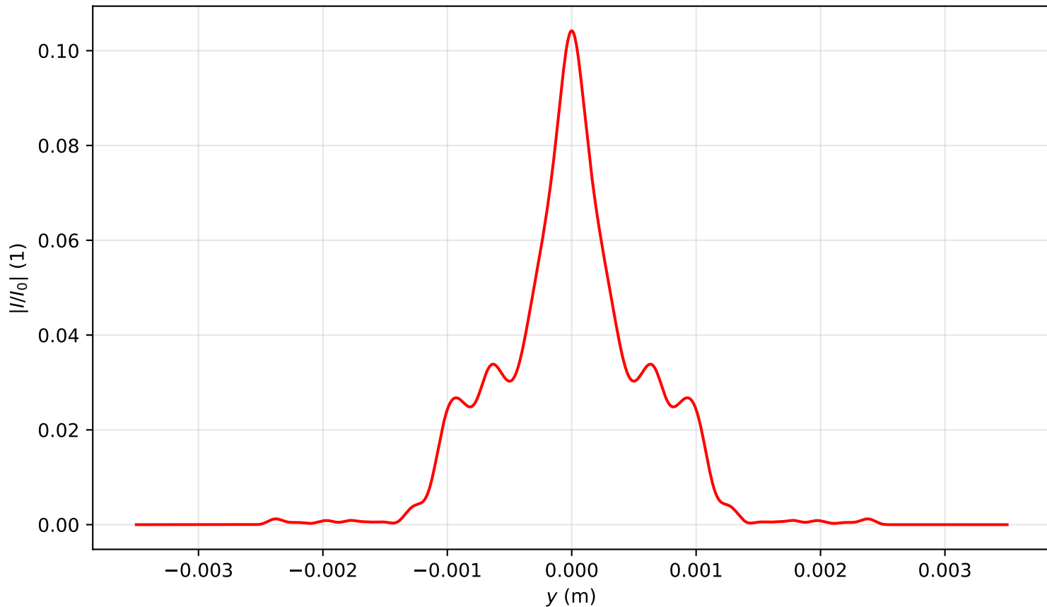
Intensity profile I(x = 0, y, z = 2.866)/I_0 , P_{in}=15.5P_{cr} , artificial time
