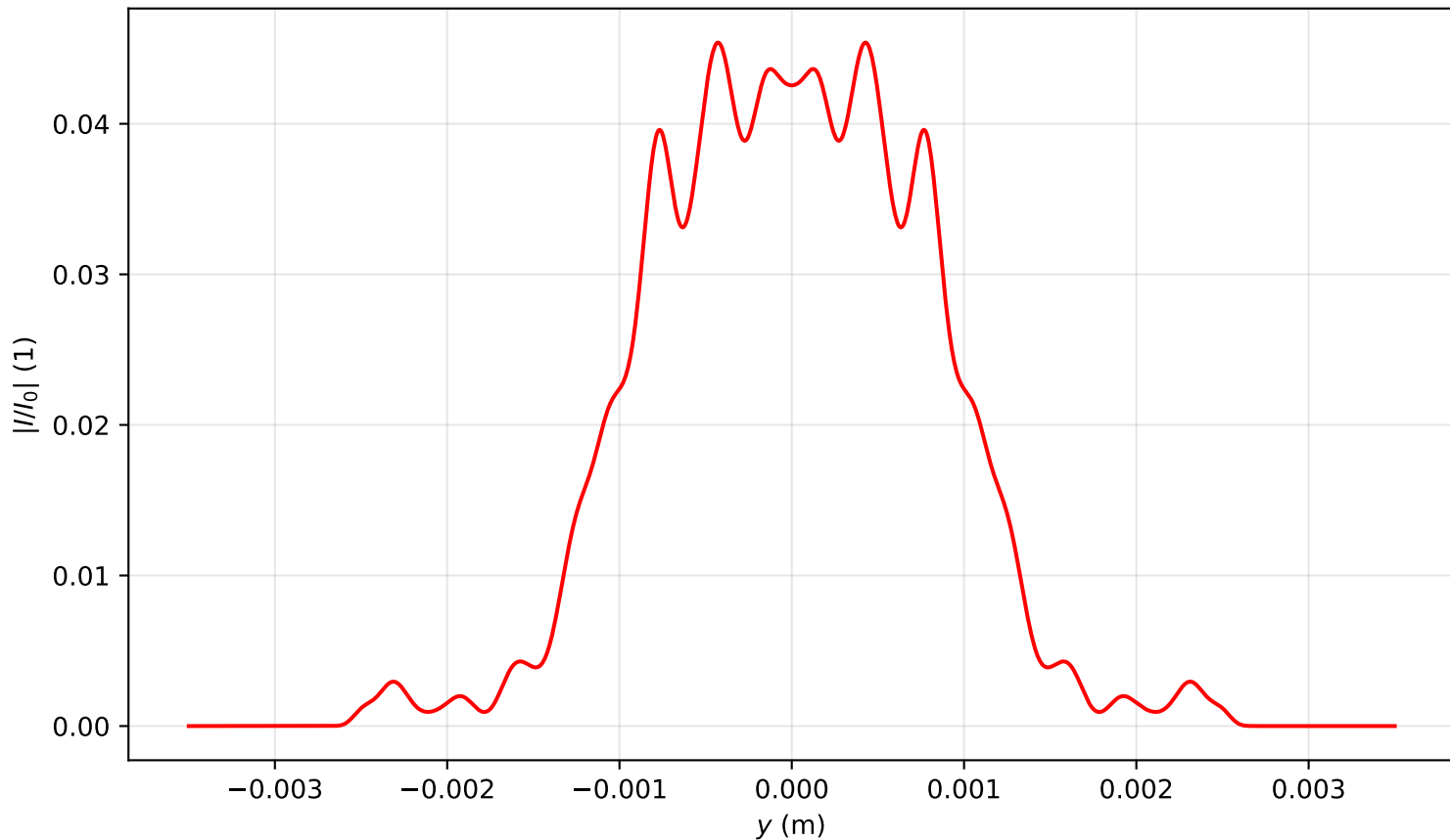
Intensity profile I(x=0, y, z=3.105)/I_0 , P_{in}=15.5P_{cr} , artificial time
