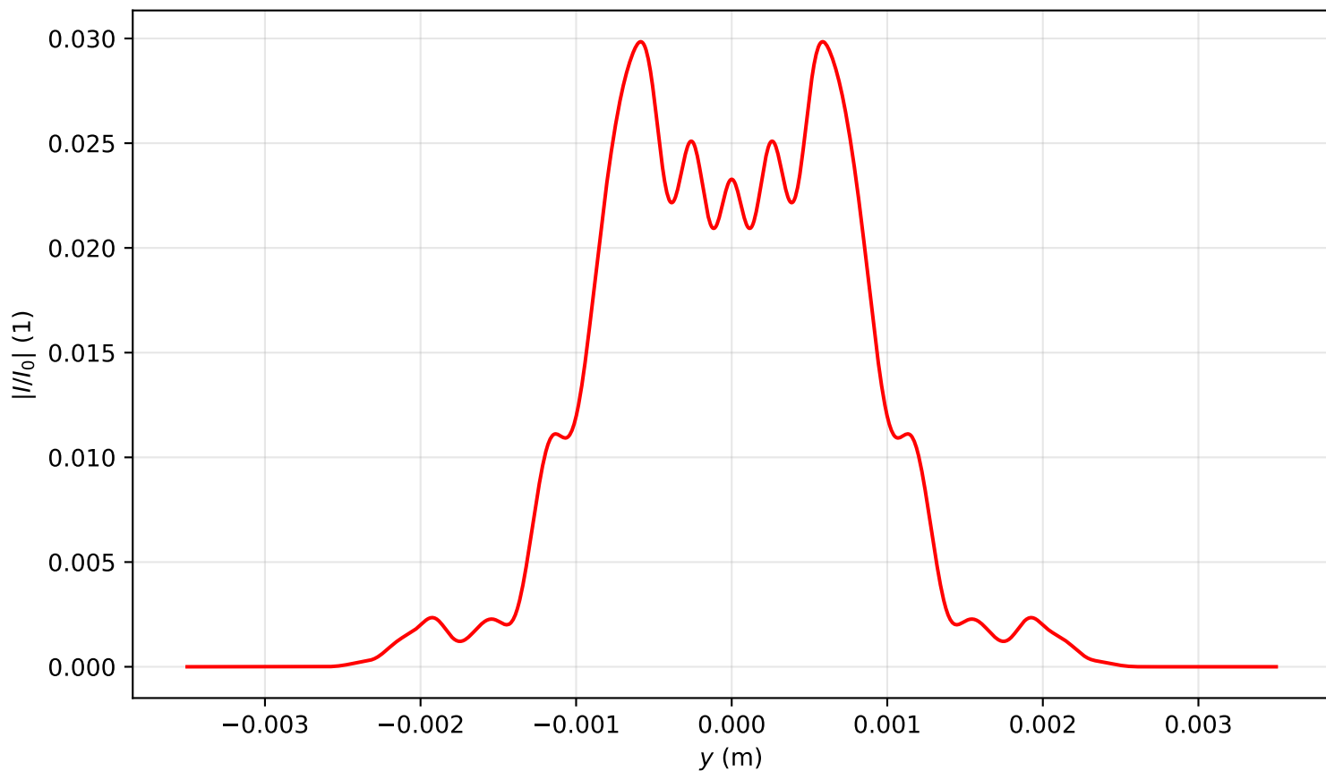
Intensity profile I(x=0, y, z=3.344)/I_0 , P_{in}=15.5P_{cr} , artificial time
