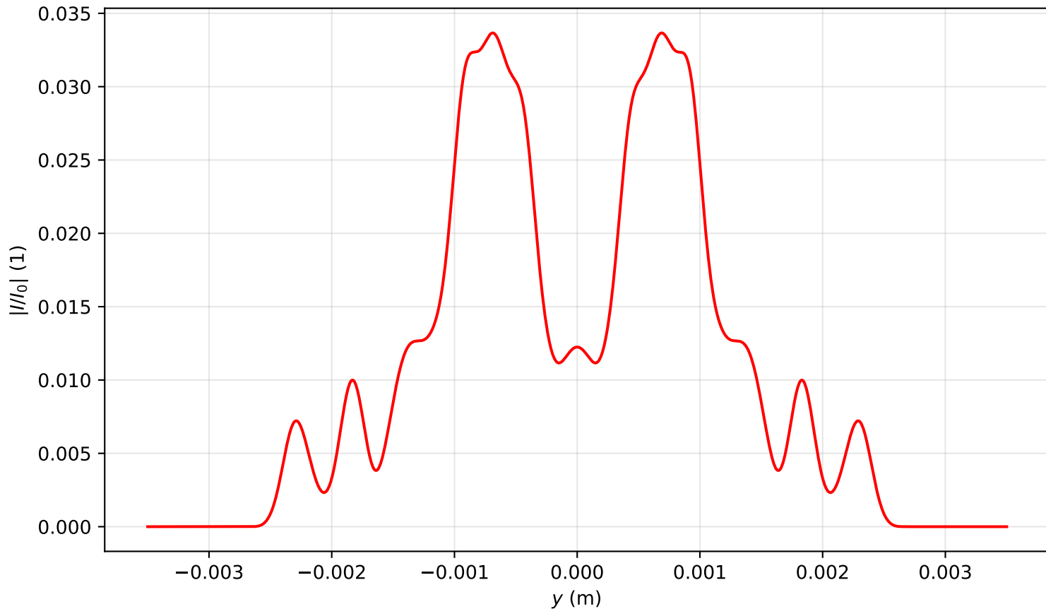
Intensity profile I(x=0, y, z=3.582)/I_0 , P_{in}=15.5P_{cr} , artificial time
