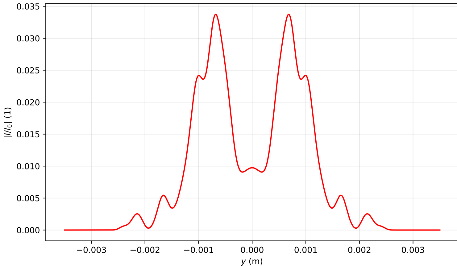
Intensity profile I(x=0, y, z=3.821)/I_0 , P_{in}=15.5P_{cr} , artificial time
