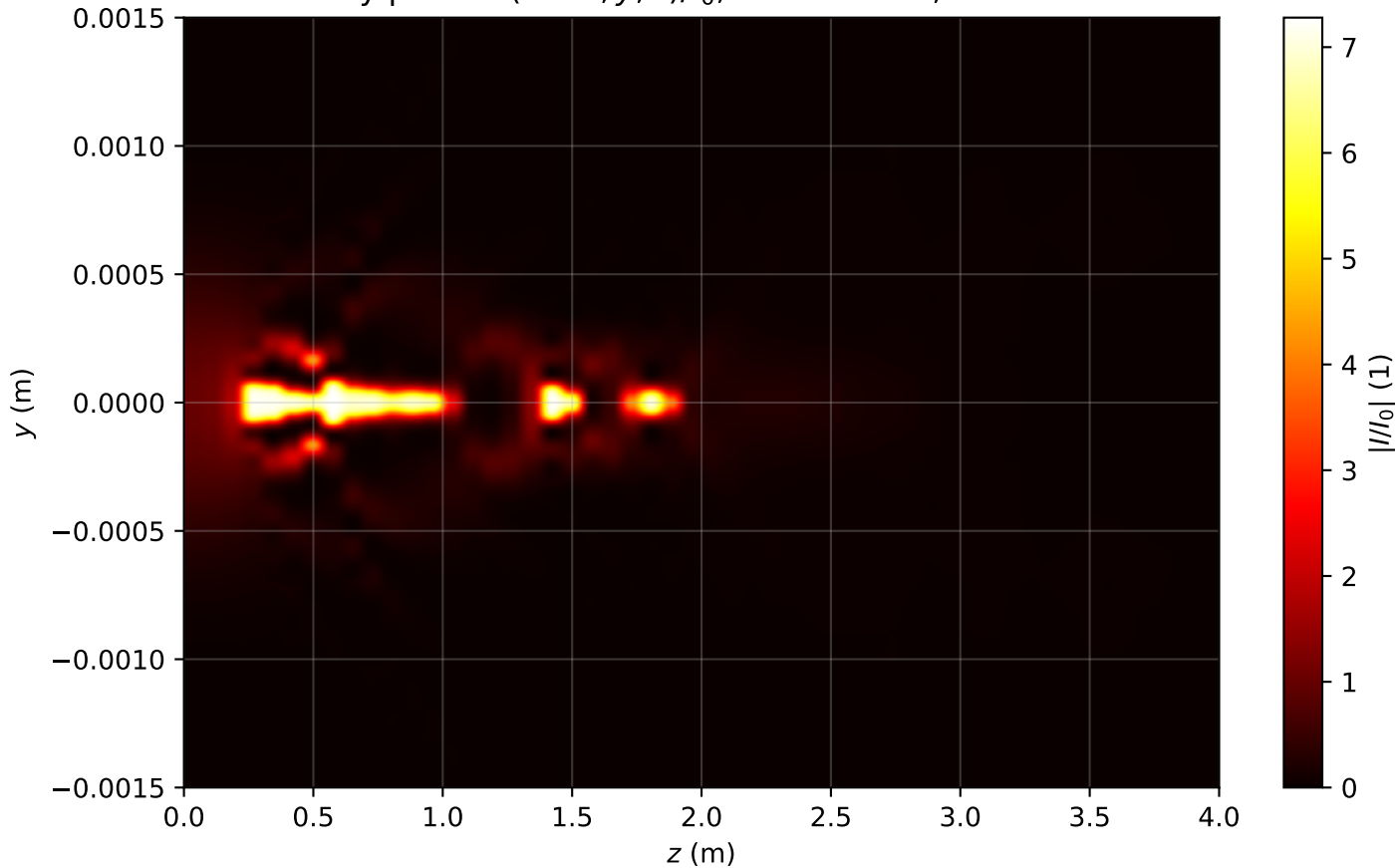
Intensity profile I(x=0, y, z)/I_0 , P_{in}=15.5P_{cr} , artificial time
