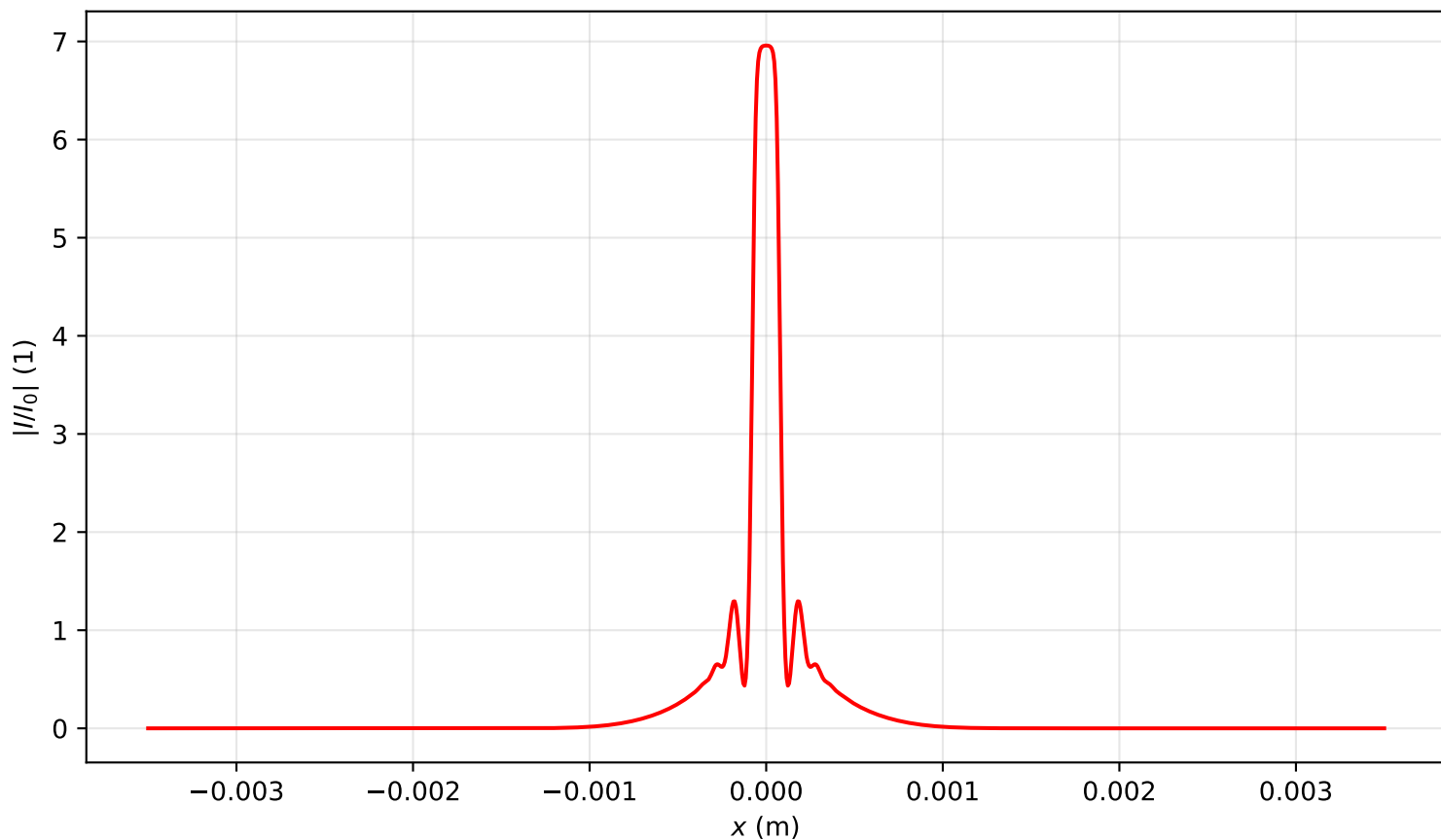
Intensity profile I(x, y = 0, z = 0.239)/I_0 , P_{in}=16.0P_{cr} , artificial time
