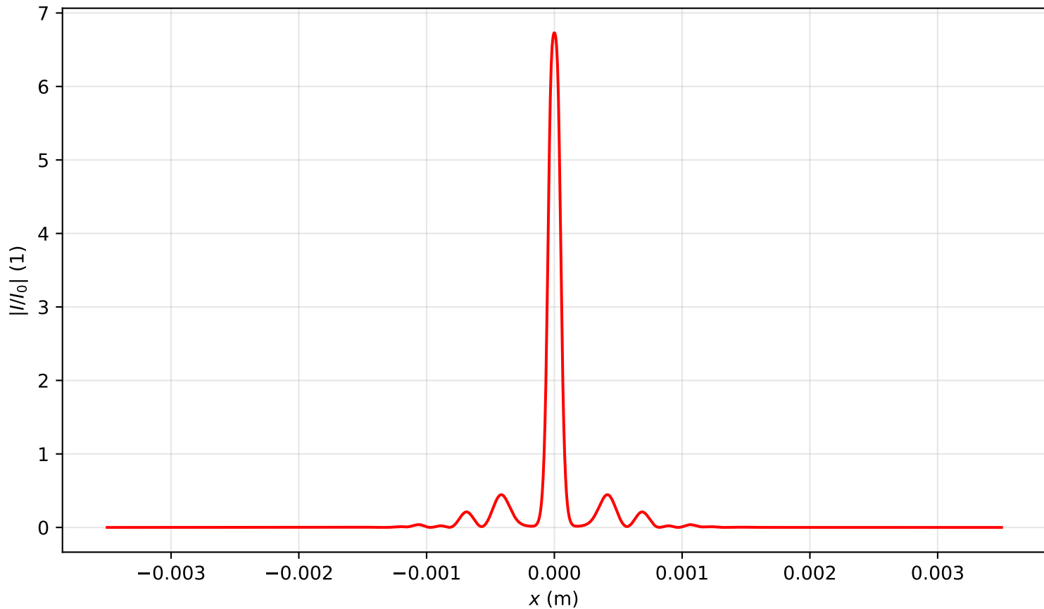
Intensity profile I(x, y = 0, z = 0.716)/I_0 , P_{in}=16.0P_{cr} , artificial time
