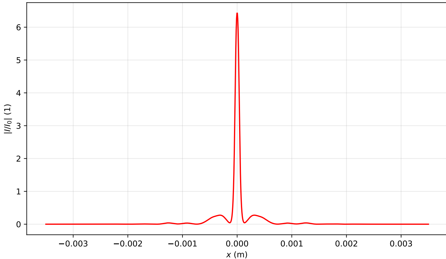
Intensity profile I(x, y = 0, z = 0.955)/I_0 , P_{in}=16.0P_{cr} , artificial time
