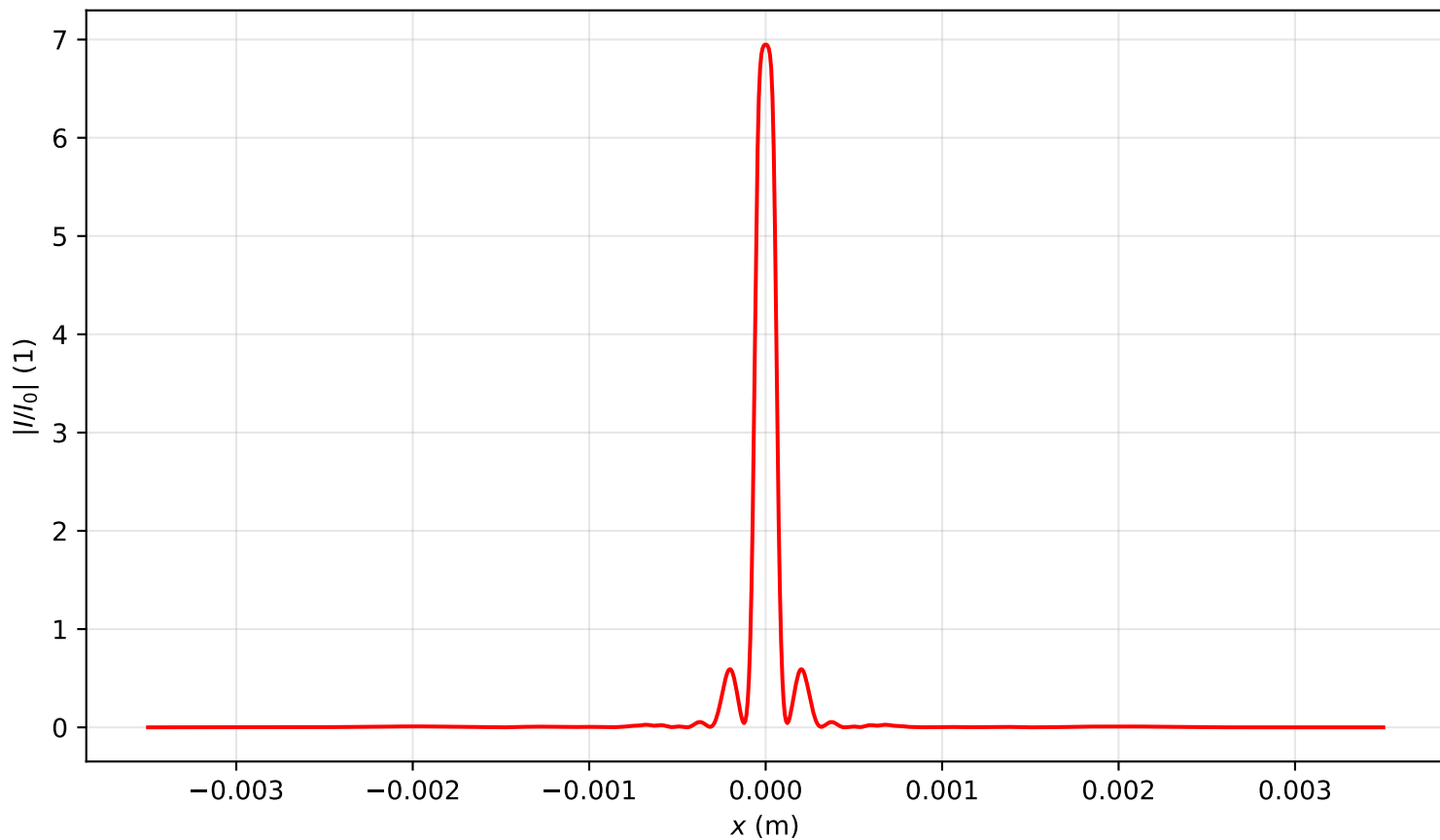
Intensity profile I(x, y = 0, z = 1.433)/I_0 , P_{in}=16.0P_{cr} , artificial time
