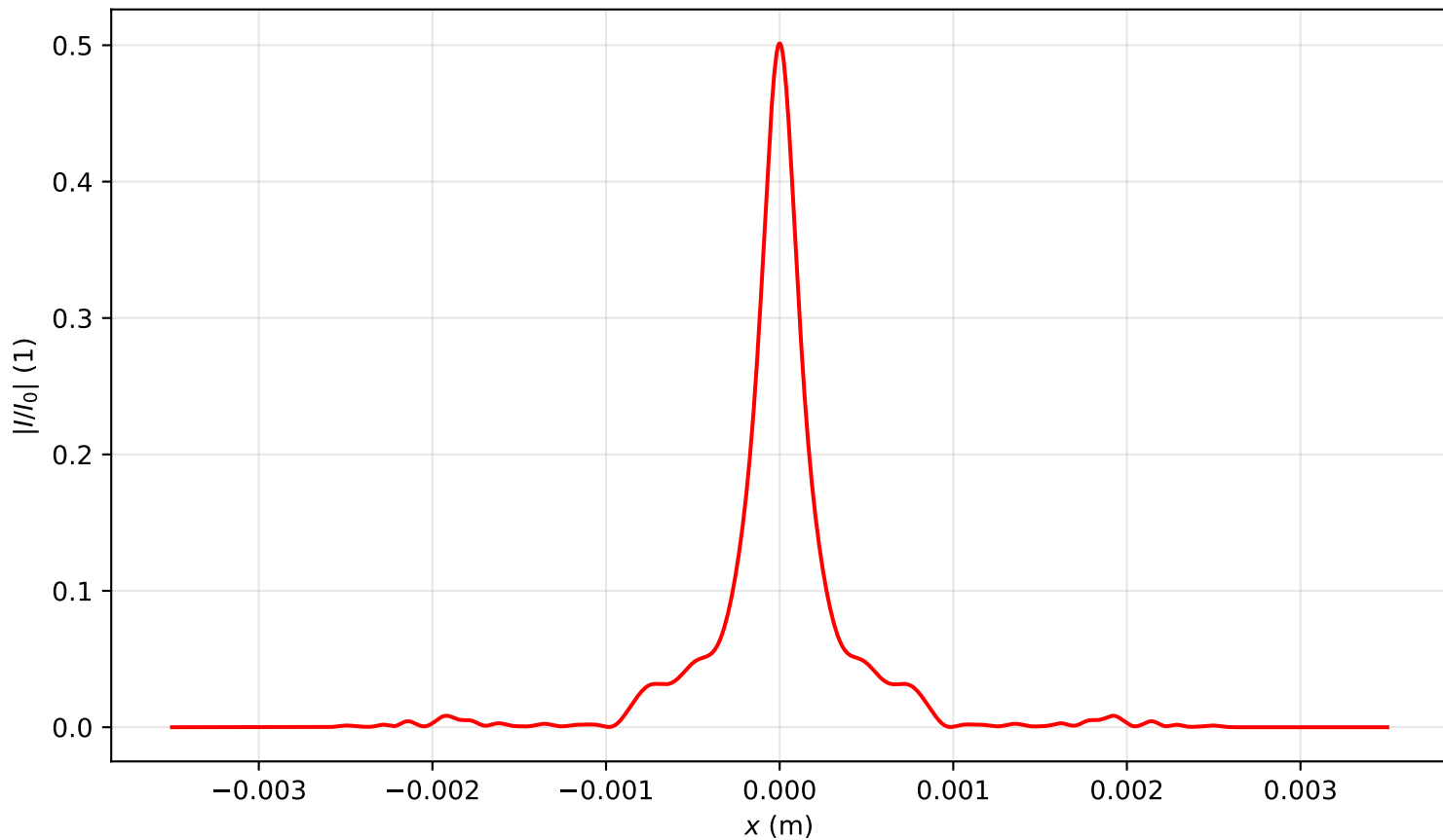
Intensity profile I(x, y = 0, z = 2.149)/I_0 , P_{in}=16.0P_{cr} , artificial time
