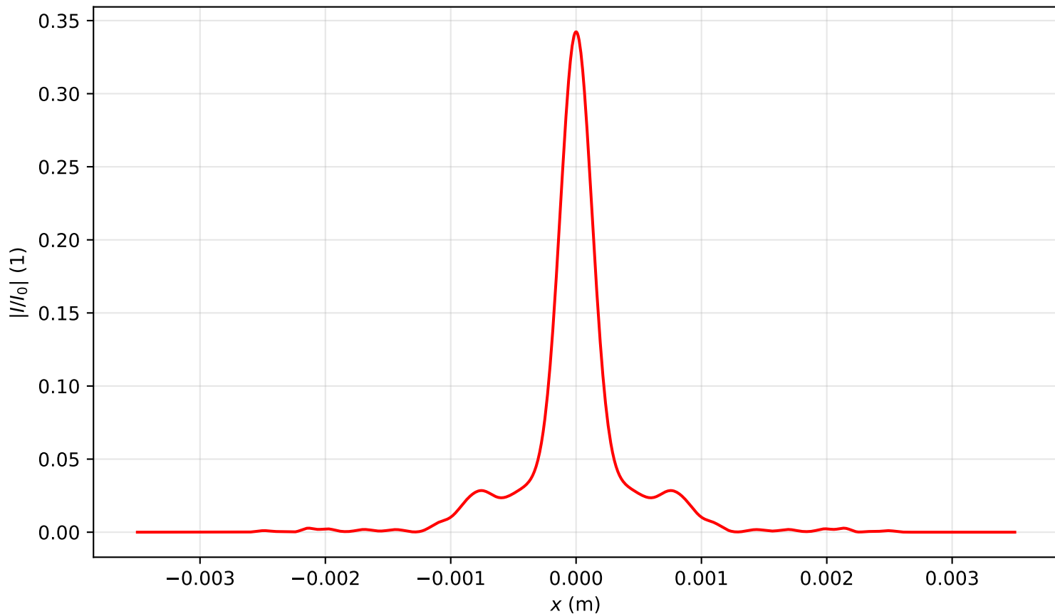
Intensity profile I(x, y = 0, z = 2.627)/I_0 , P_{in}=16.0\text{Pcr} , artificial time
