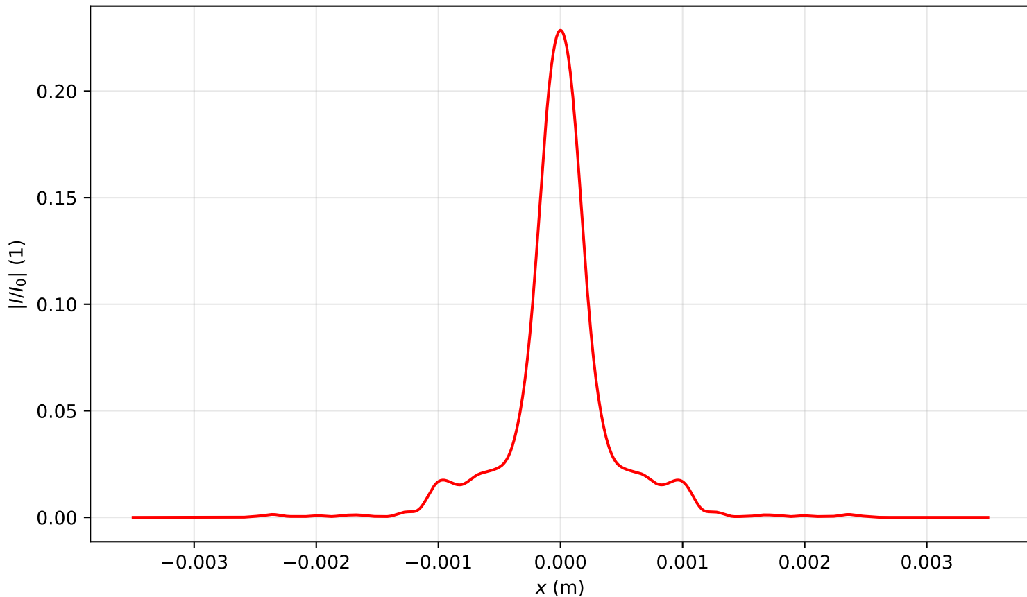
Intensity profile I(x, y = 0, z = 2.866)/I_0 , P_{in}=16.0P_{cr} , artificial time
