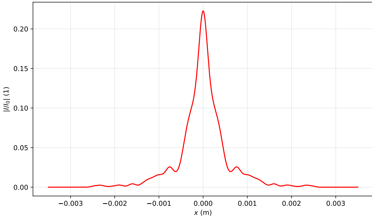
Intensity profile I(x, y = 0, z = 3.105)/I_0 , P_{in}=16.0P_{cr} , artificial time
