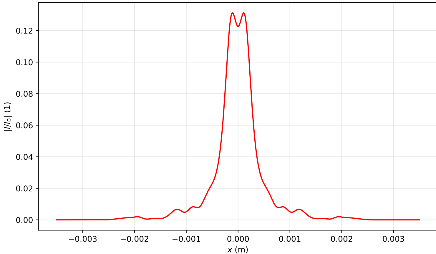
Intensity profile I(x, y = 0, z = 3.344)/I_0 , P_{in}=16.0P_{cr} , artificial time
