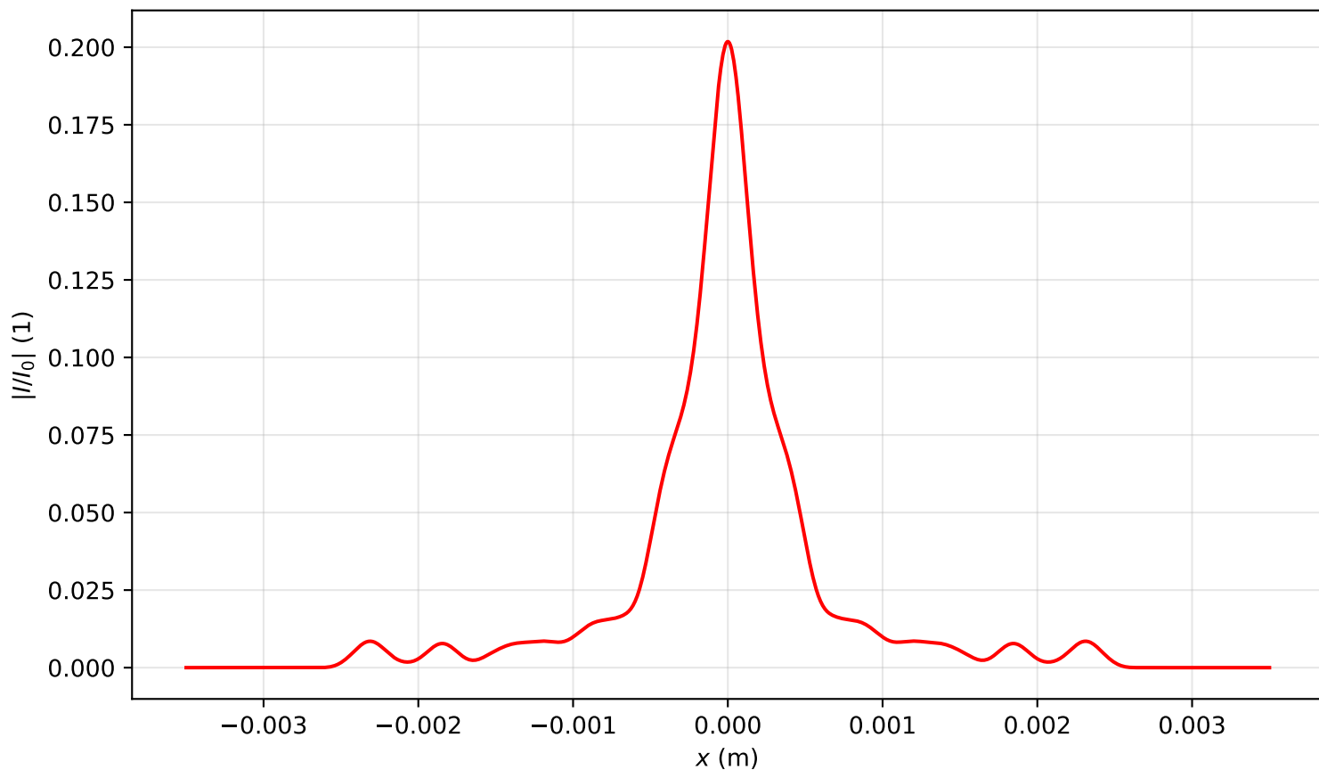
Intensity profile I(x, y = 0, z = 3.582)/I_0 , P_{in}=16.0P_{cr} , artificial time
