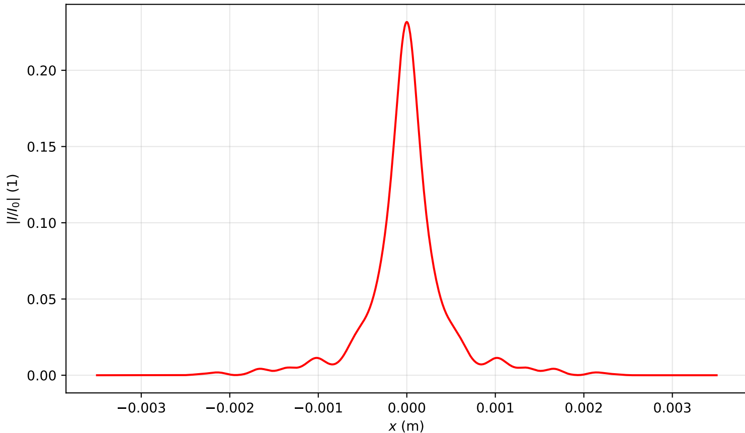
Intensity profile I(x, y = 0, z = 3.821)/I_0 , P_{in}=16.0P_{cr} , artificial time
