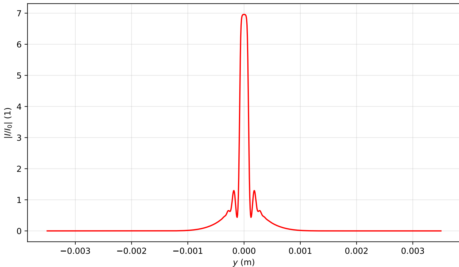
Intensity profile I(x=0, y, z=0.239)/I_0 , P_{in}=16.0P_{cr} , artificial time
