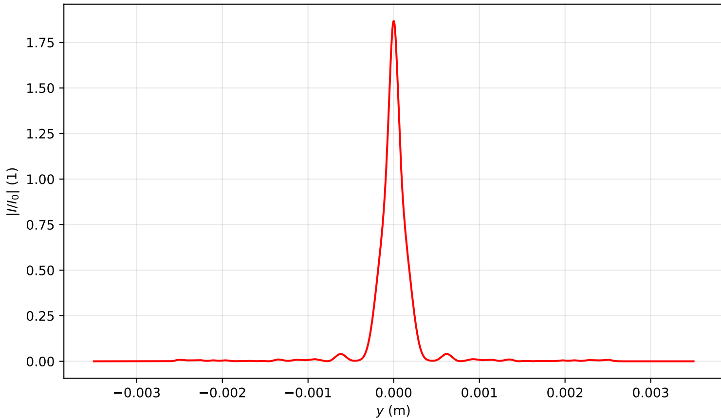
Intensity profile I(x=0, y, z=1.672)/I_0 , P_{in}=16.0P_{cr} , artificial time
