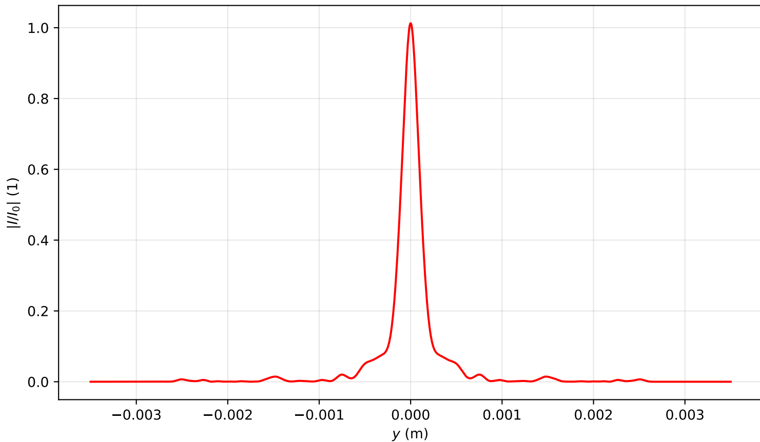
Intensity profile I(x=0, y, z=1.911)/I_0 , P_{in}=16.0P_{cr} , artificial time
