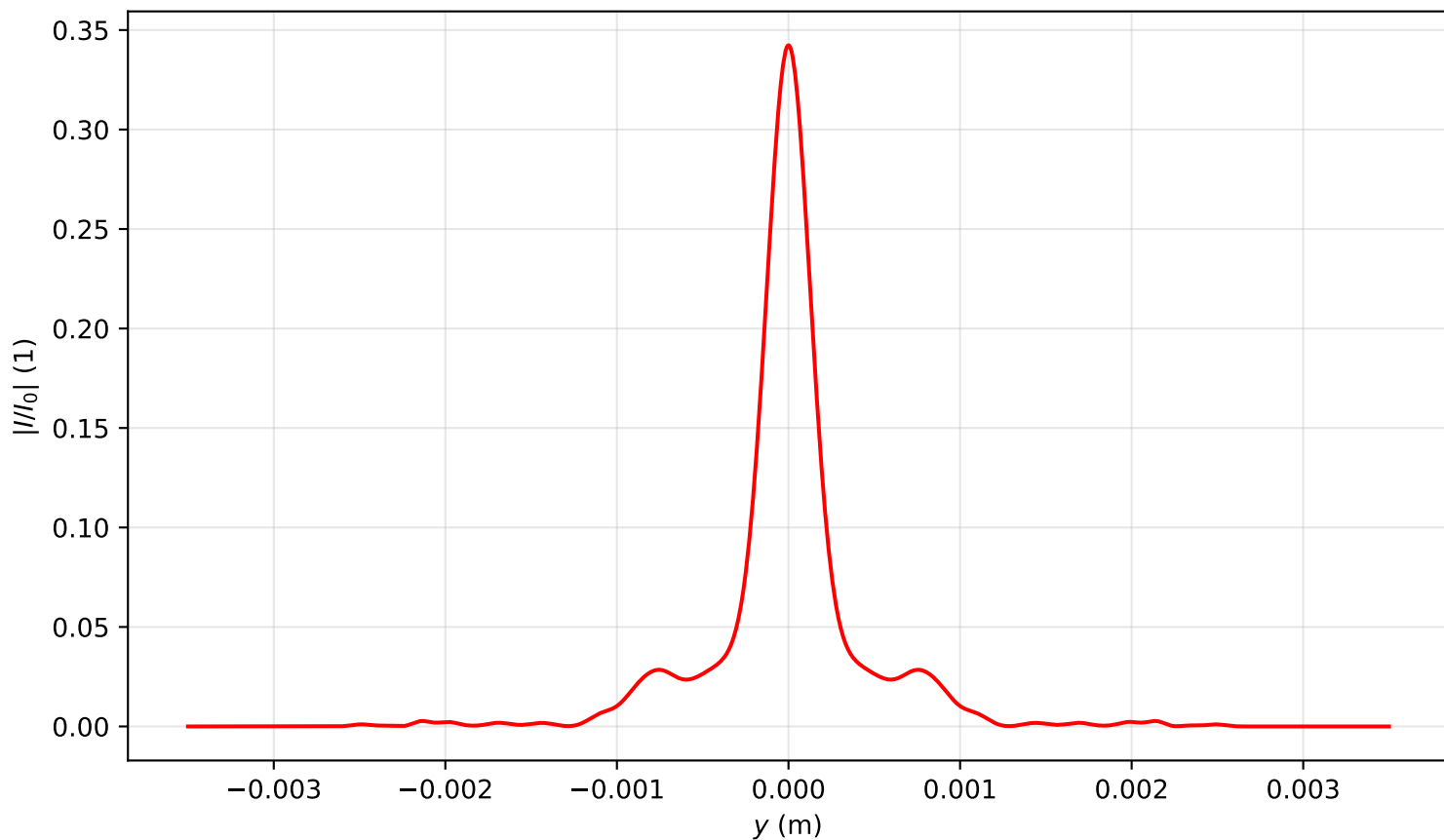
Intensity profile I(x = 0, y, z = 2.627)/I_0 , P_{in}=16.0P_{cr} , artificial time
